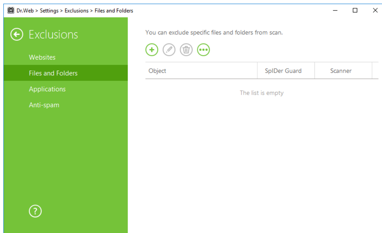
Figure 36. Excluding files and folders from scanning
