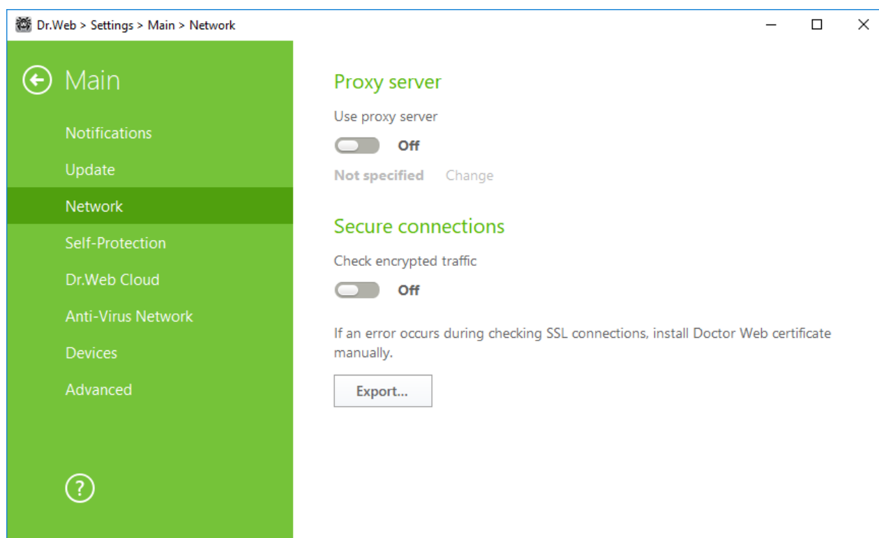
Figure 24. Connecting to proxy server and checking the encrypted traffic
