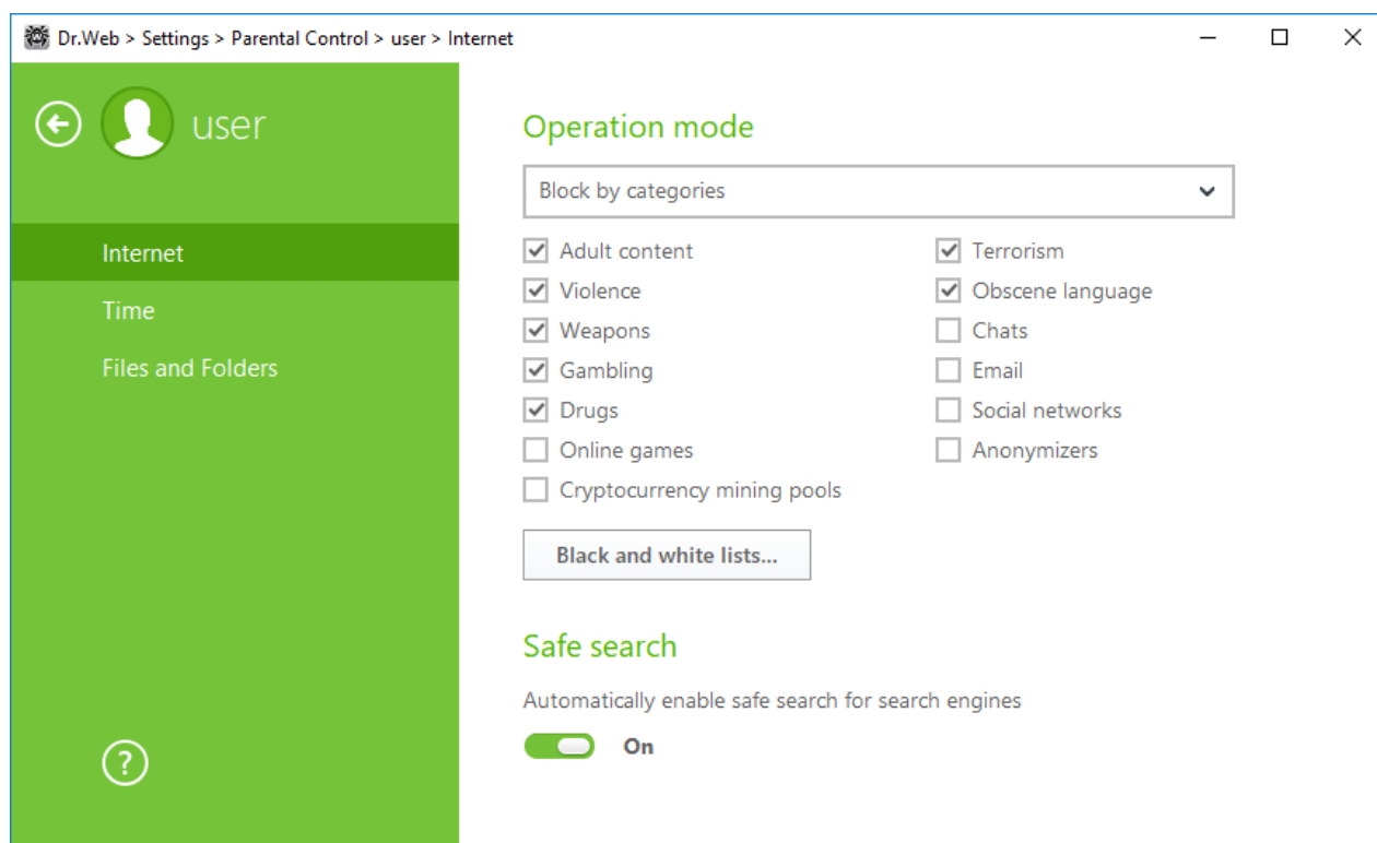
Figure 31. Managing the Internet access by websites categories
