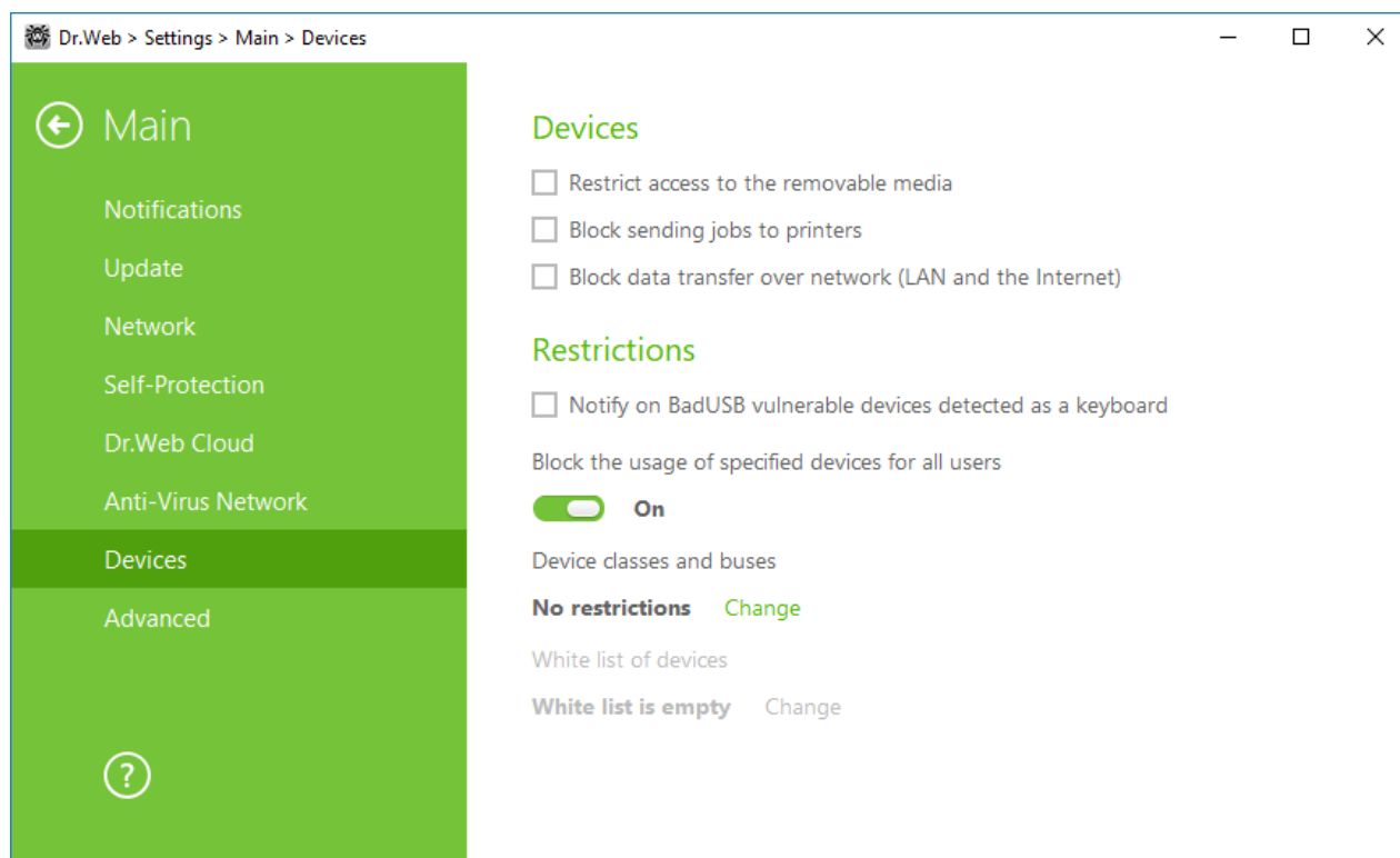
Figure 28. Devices lock settings
