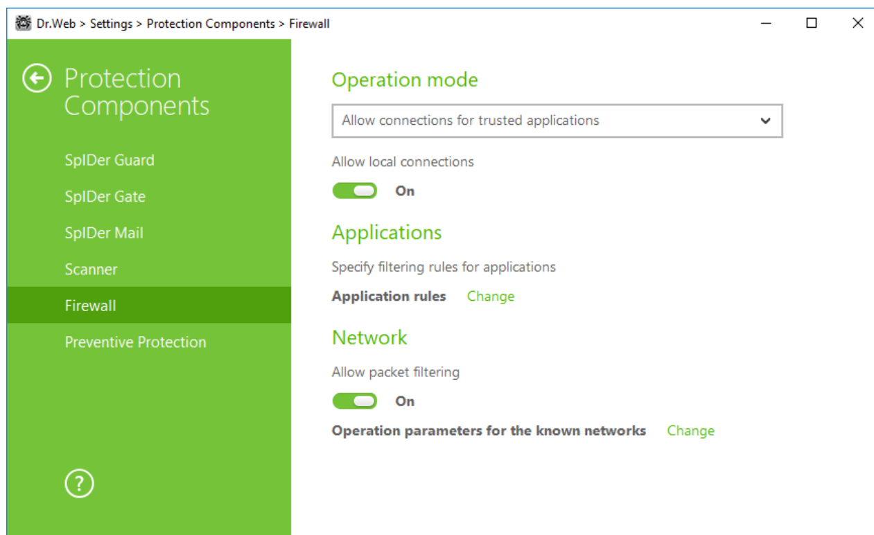
Figure 44. Firewall main settings
